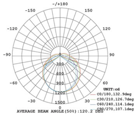
E-B40W-CC | 5700K
