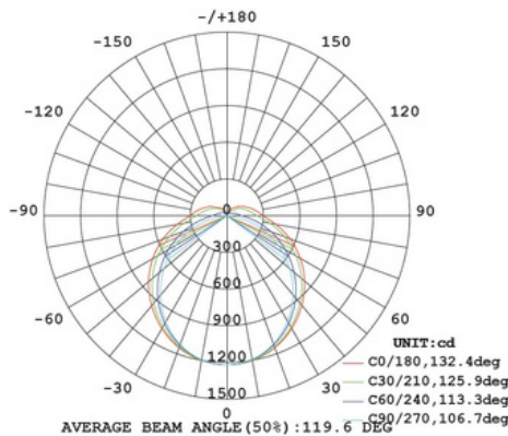
E-B40W-CC | 4000K
