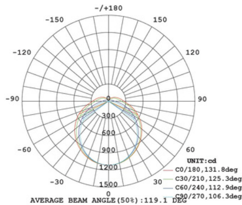
E-B40W-CC | 3000K
