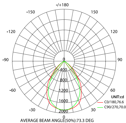
SL32W-CC | 5700K
