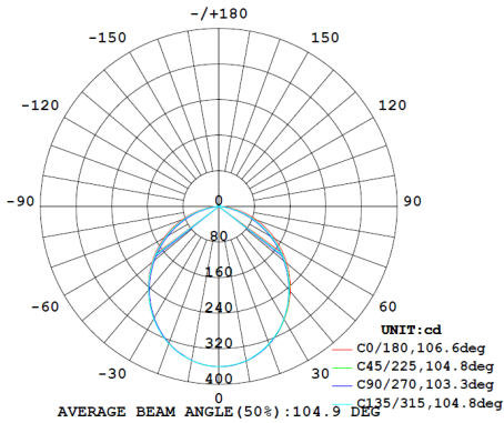
IDI10WCOB-CC | 3000K
