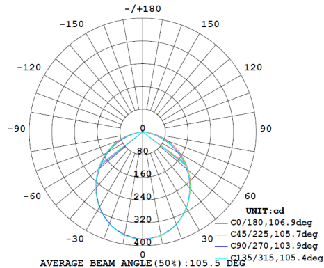
IDI10WCOB-CC | 5700K
