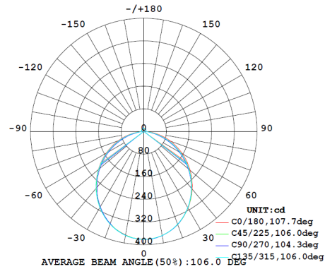
IDI10WCOB-CC | 4000K
