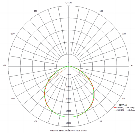
UFO-200W-E-170LM | 200W
