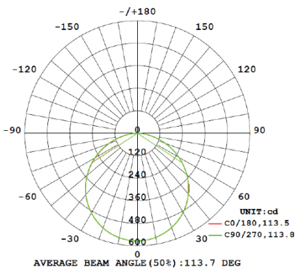
BLP16W-30/60 | 5700K
