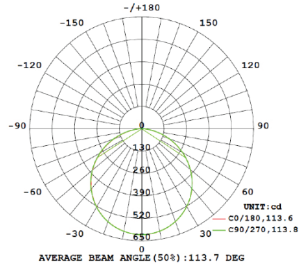
BLP16W-30/60 | 4000K
