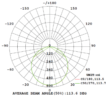
BLP16W-30/60 | 3000K
