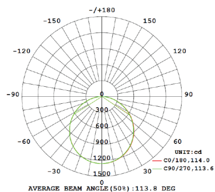
BLP36W-60SQ | 5700K
