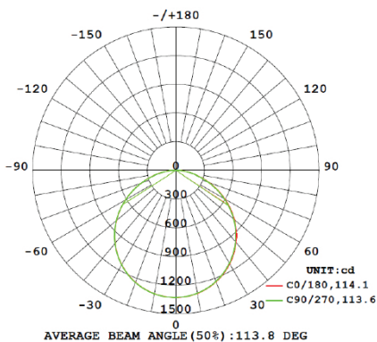
BLP36W-60SQ | 4000K
