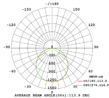
BLP36W-60SQ | 3000K
