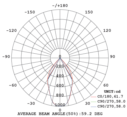
LED-DL13WCOB-CC | 5000K
