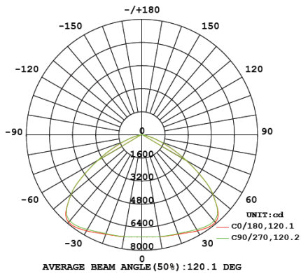
HBI20-200W | 120W
