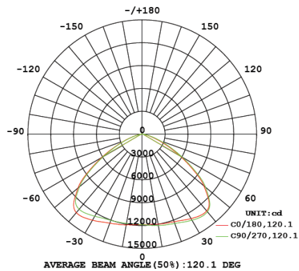
HBI20-200W | 200W
