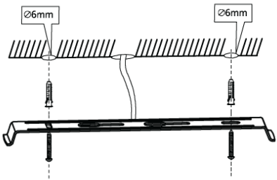
Fig 2. Fix the mounting bracket to the wall/ ceiling.
