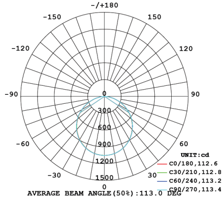
LED-LPE28W-60SQ | 4000K
