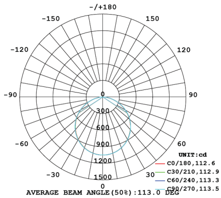
LED-LPE28W-120/30 | 4000K
