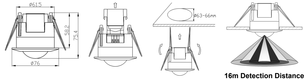
16m Detection Distance
