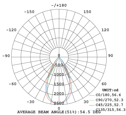
CD25W-CC | 5000K
