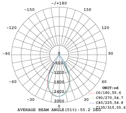
CD25W-CC | 4000K
