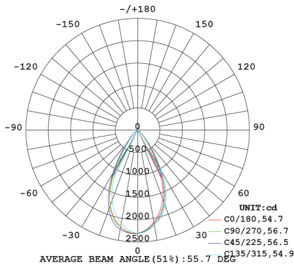
CD25W-CC | 3000K
