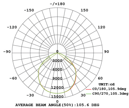
UFO-200W-E-I70LM | 6000K
