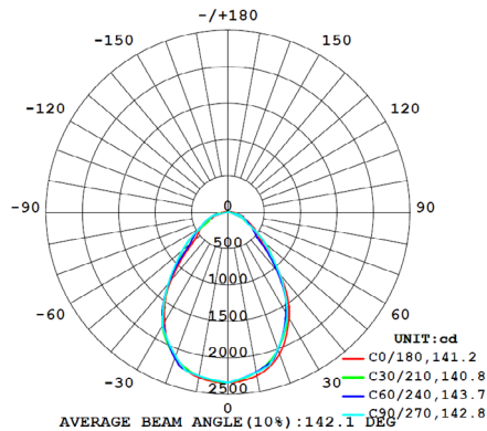
LED-CLP48W-120/60 | 4000K
