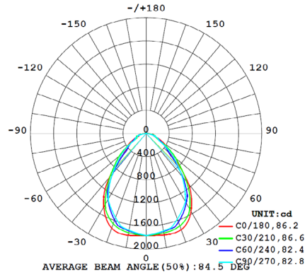
LED-CLP36W-60SQ | 4000K
