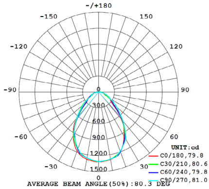
LED-CLP25W-30/60 | 4000K
