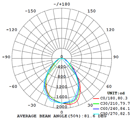
LED-CLP36W-120/30 | 4000K
