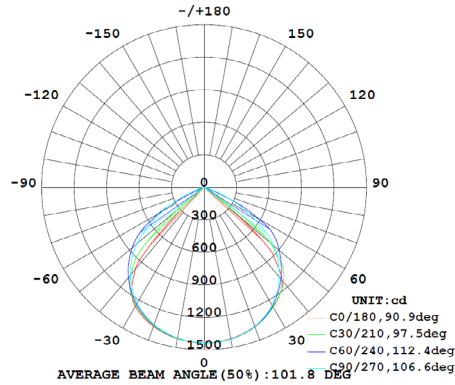
LED-SL35W-CW | 5700K
