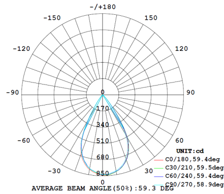
DL10WCOB-G | 4000K
